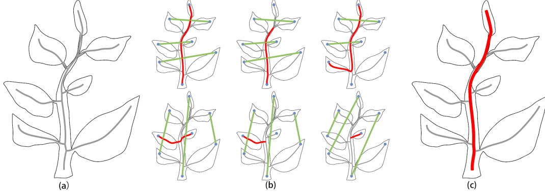
Figure 2: Backbone detection: given a shape with an automatically extracted skeleton (a), red curves in (b) represent some potential backbone candidates, where green lines denote the established self-matching between end nodes (blue dots) about the candidate; the red path in (c) is our detected backbone with the optimal self-matching.
